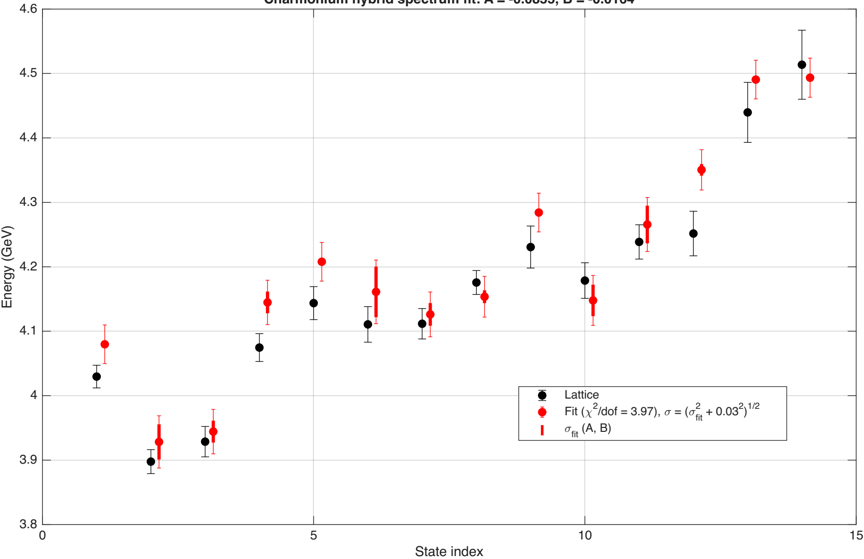
Charmonium hybrid spectrum fit: A = -0.0855, B = -0.0164
